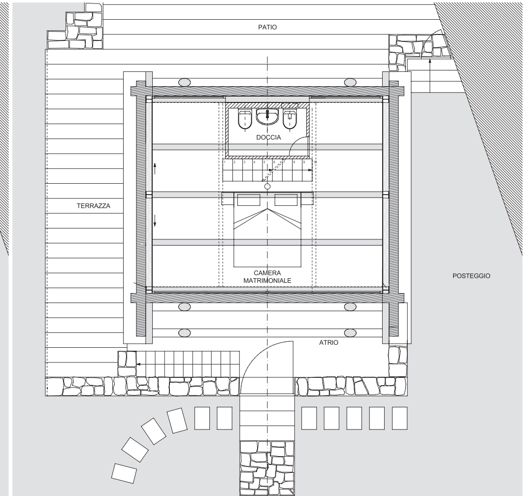
PIANTA PIANO MANSARDA
